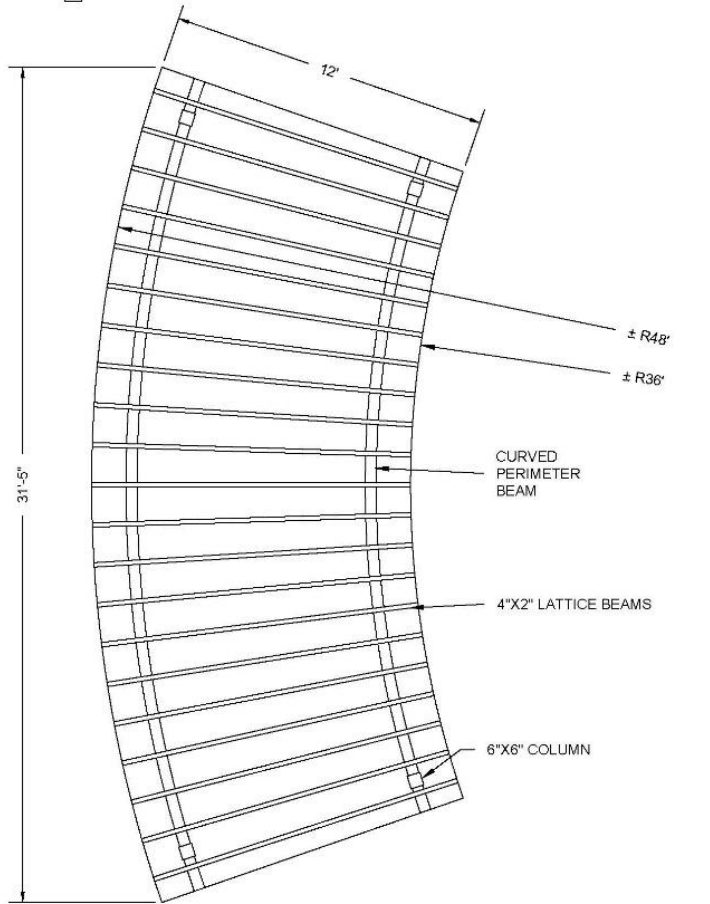
PLAN VIEW 12'X31'-5" CURVED TRELLIS MODEL NTS
