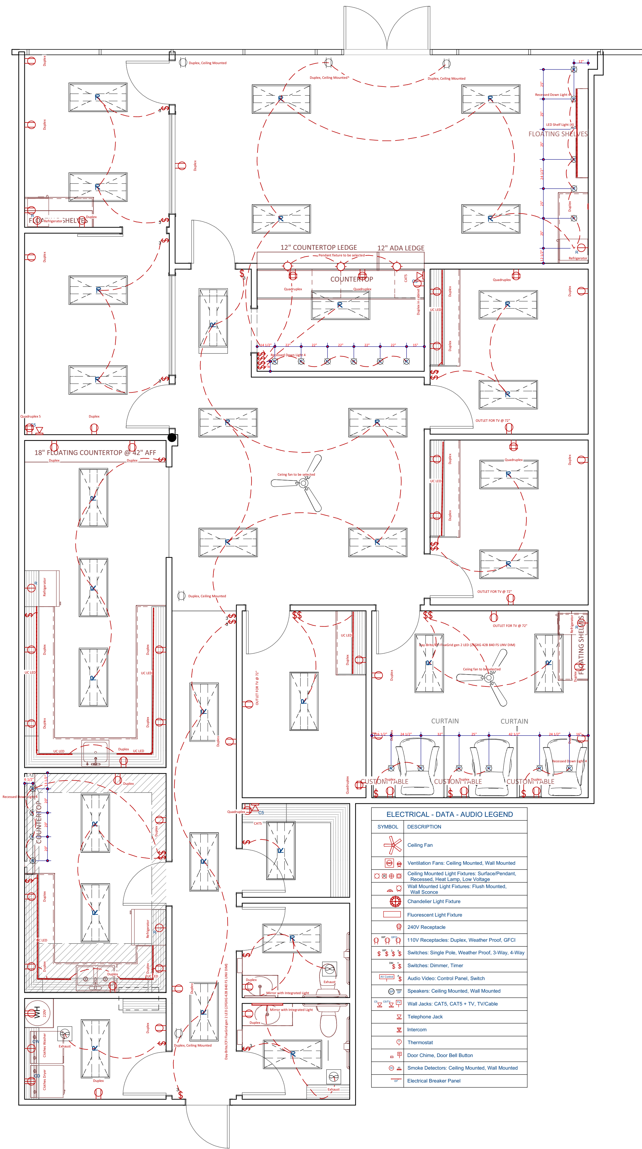
01 ELECTRICAL PLAN SCALE: 1/4" = 1'-0"
