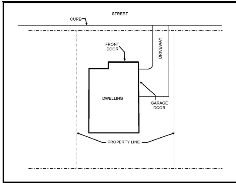
Figure 24 - Side Entry Garage
