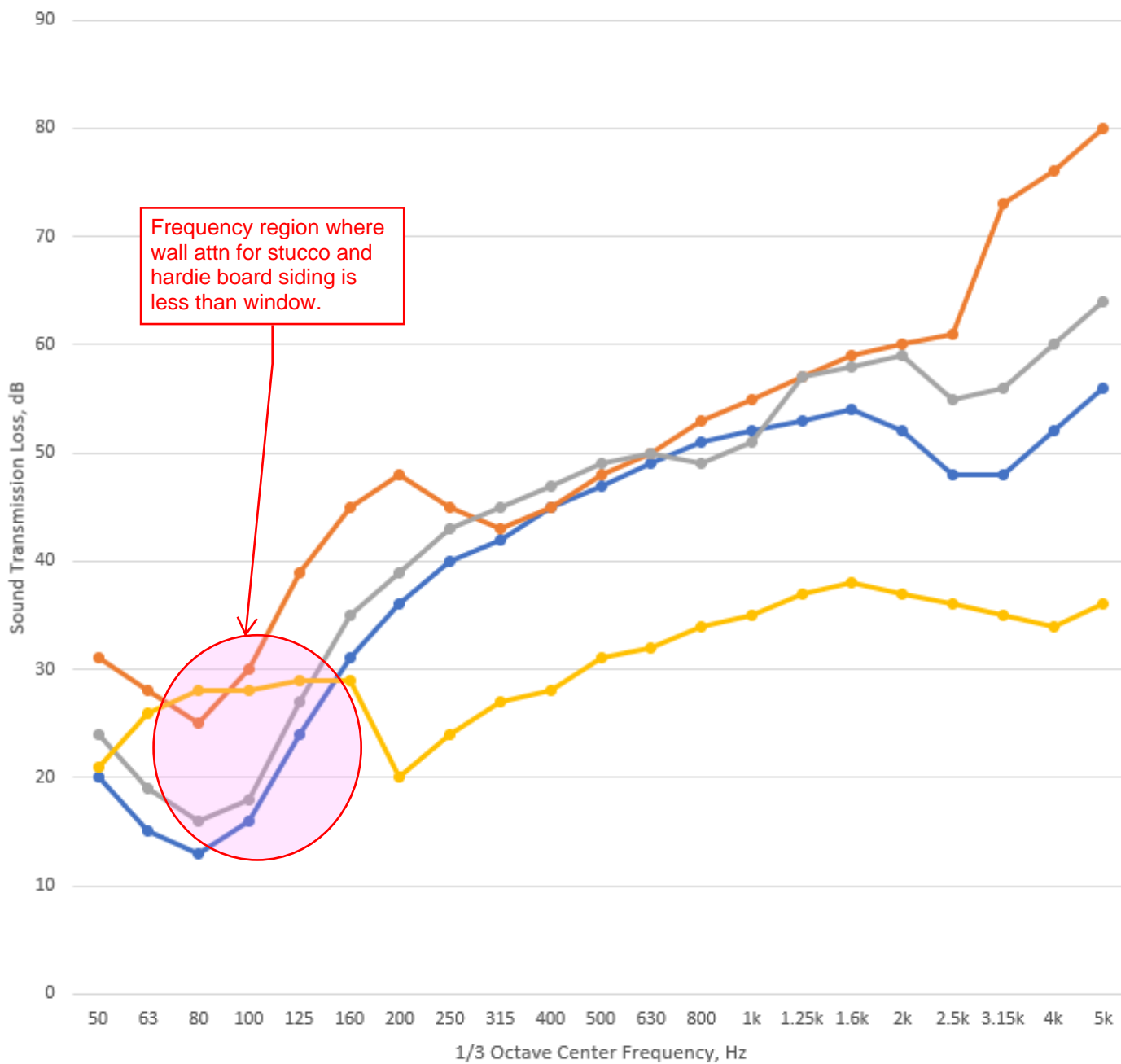
Graph 4 Sound Transmission Loss Comparison of Different Ext Wall Assemblies
