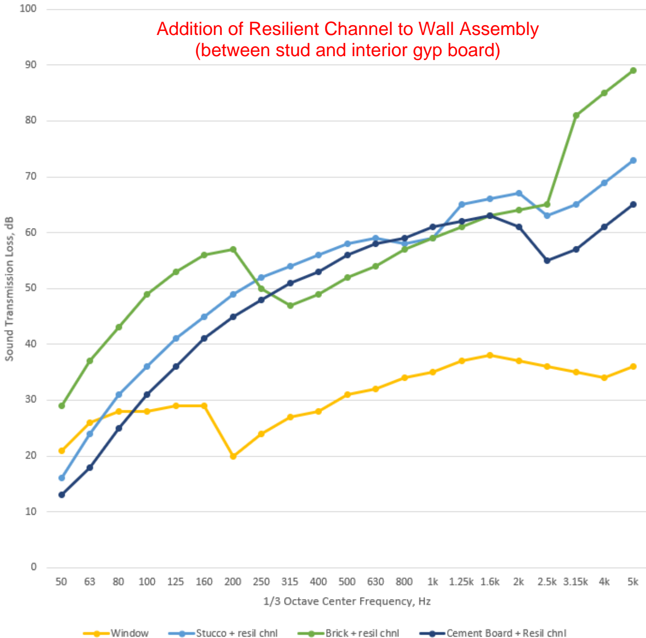
Graph 5 Sound Transmission Loss Comparison of Different Ext Wall Assemblies
