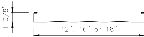
PLANK PROFILE
