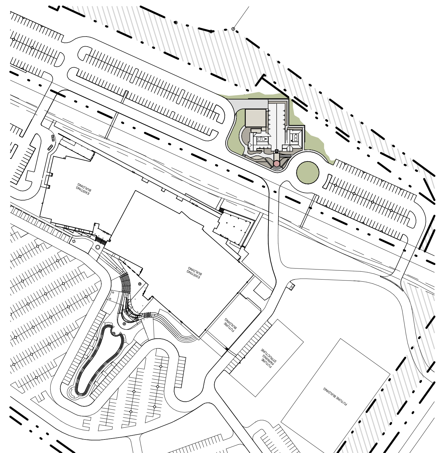
2 OVERALL SITE A110 1" = 160'-0"
