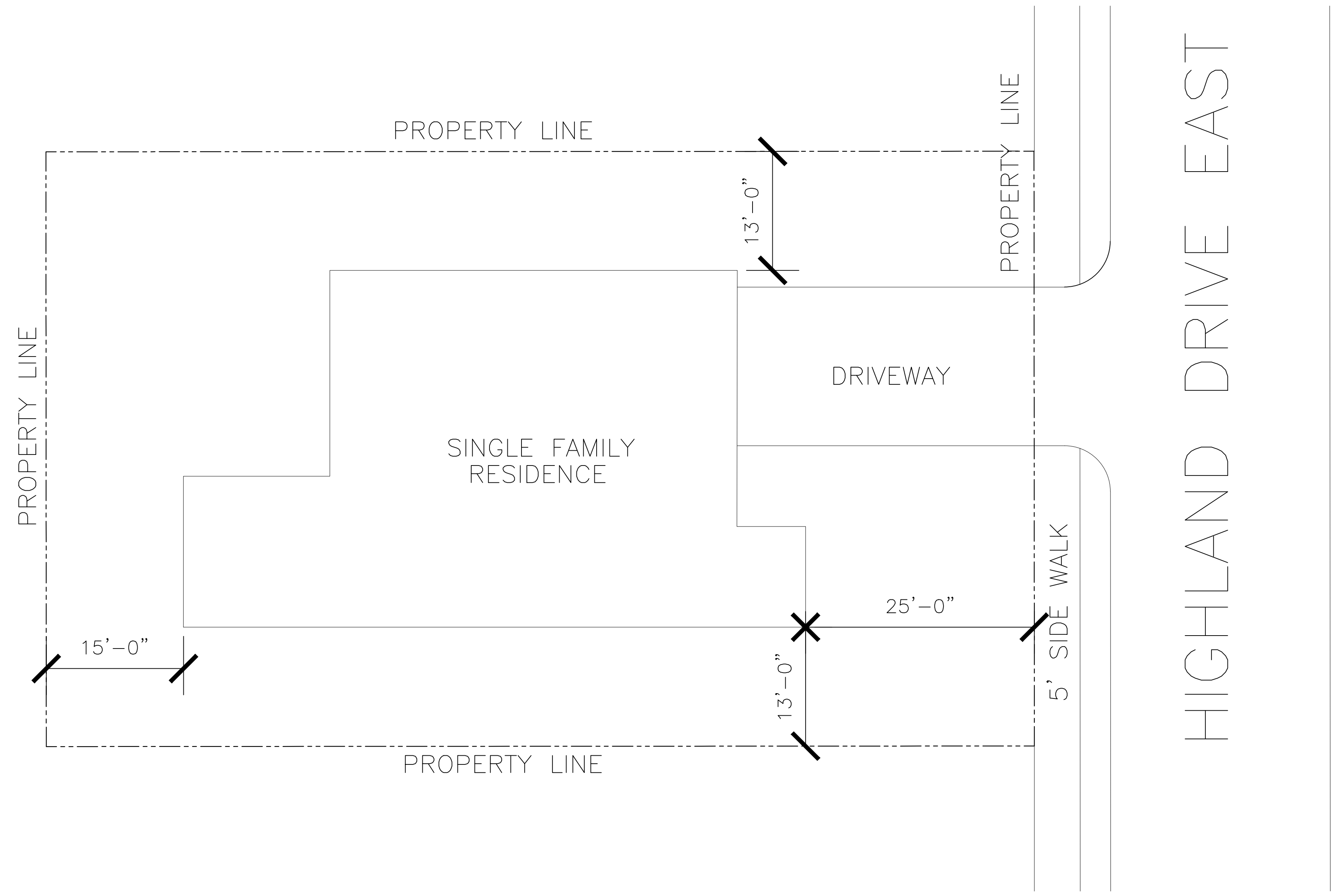
1 SITE PLAN SCALE 1/8"=1'-0"
