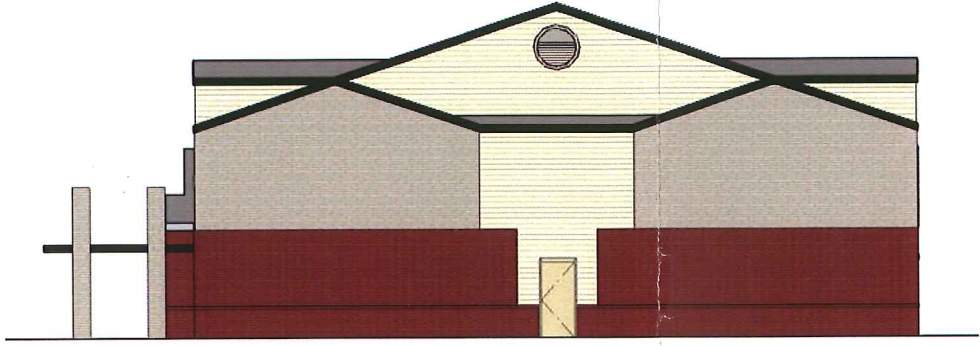
2 FIRE STATION ELEVATION - PLAN EAST SCALE: 1/8" = 1'-0"
