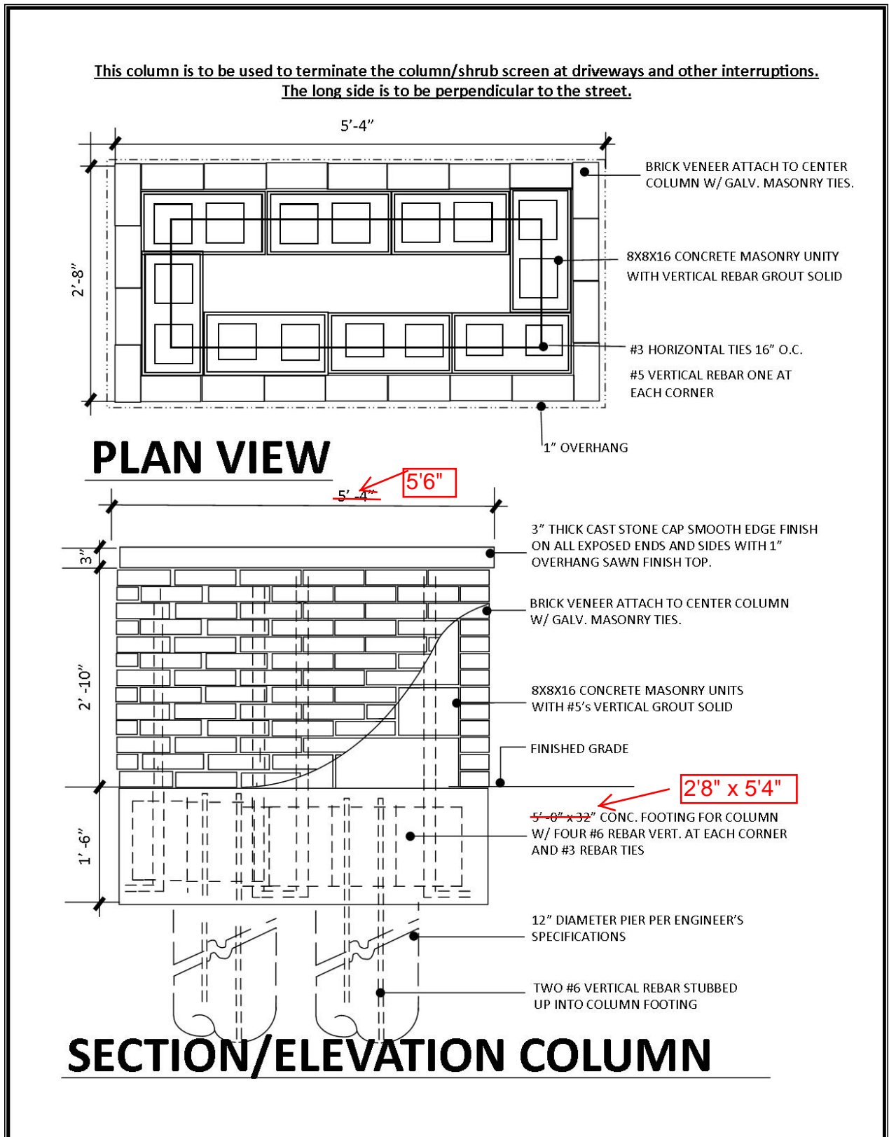
Figure 19 – Brick Columns Details
