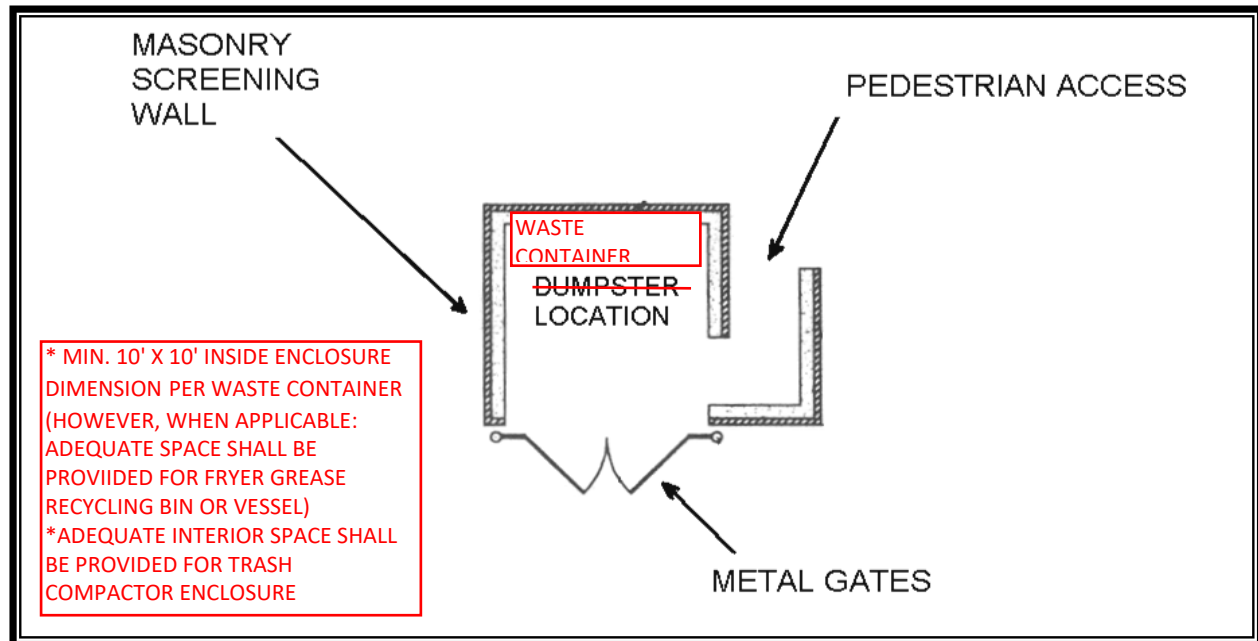
Figure 20 - Pedestrian Access for Typical Waste Container Screening Closure
